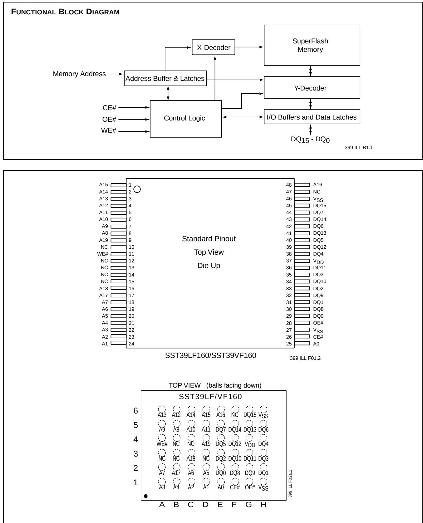
FIGURE 1: PIN ASSIGNMENTS FOR 48-LEAD TSOP AND 48-BALL TFBGA
