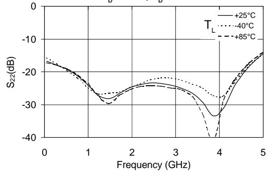
S_{22} vs. Frequency V_D = 2.2 V, I_D = 20 mA
