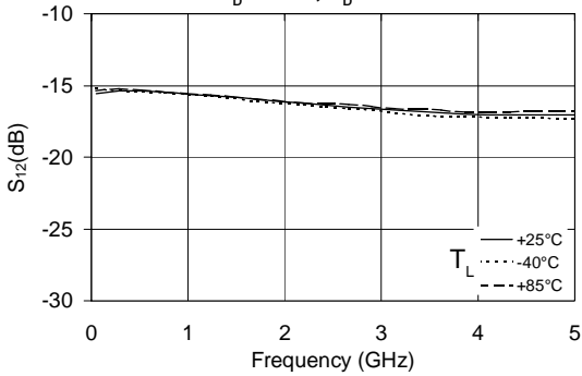
S_{12} vs. Frequency V_D = 2.2 V, I_D = 20 mA
