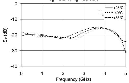
S_{11} vs. Frequency V_D = 2.2 V, I_D = 20 mA
