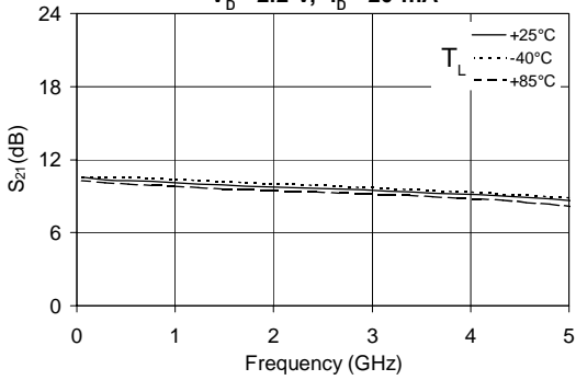
S_{21} vs. Frequency V_D = 2.2 V, I_D = 20 mA
