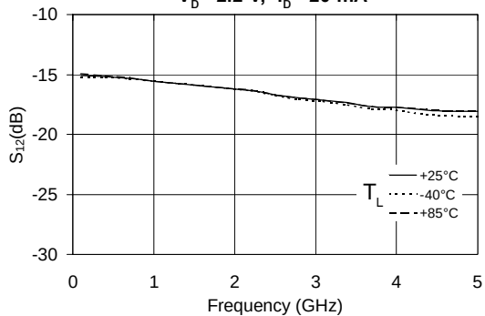
S_{12} vs. Frequency V_D = 2.2 \text{ V} , I_D = 20 \text{ mA}
