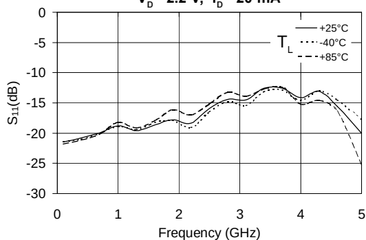
S_{11} vs. Frequency V_D = 2.2 \text{ V} , I_D = 20 \text{ mA}
