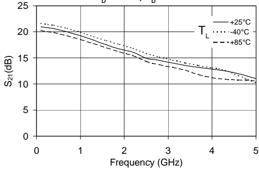
S_{21} vs. Frequency V_D = 2.7 V, I_D = 20 mA
