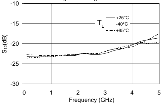
S_{12} vs. Frequency V_D = 2.7 V, I_D = 20 mA
