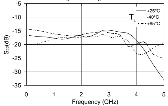
S_{22} vs. Frequency V_D = 2.7 V, I_D = 20 mA
