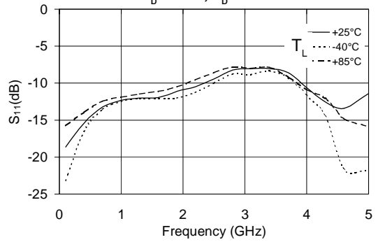
S_{11} vs. Frequency V_D = 2.7 V, I_D = 20 mA
