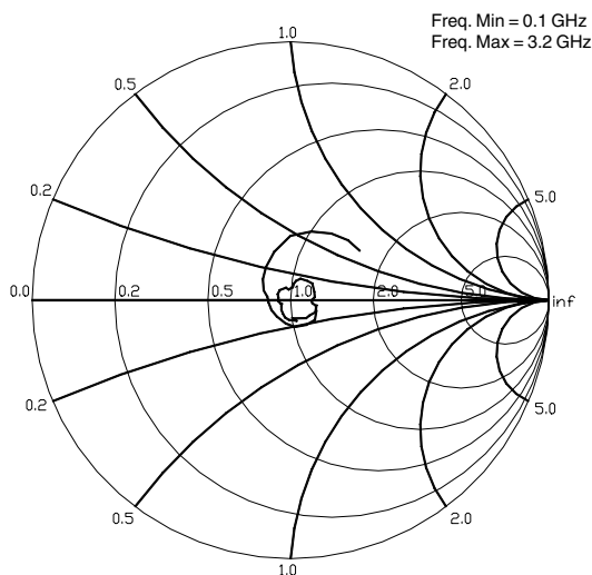
S22, Id=60mA, Ta= 85C
