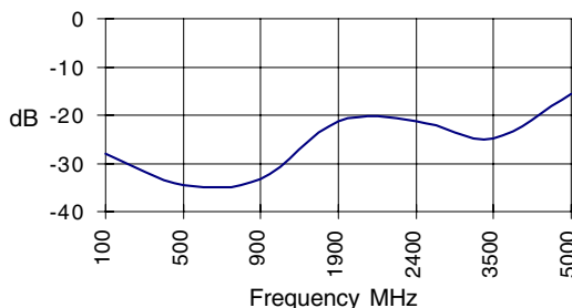
S22, Id =60mA, T=85C
