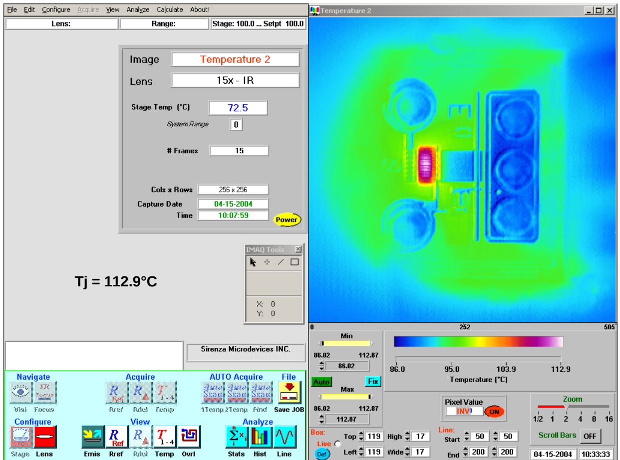
Figure 2: Infrared Thermal Image of SGA-8343X, Vd =4V, Id =50 mA, T lead = 85°C
