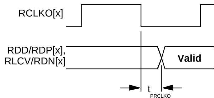
Figure 35 - RCLKO Output Timing Diagram
