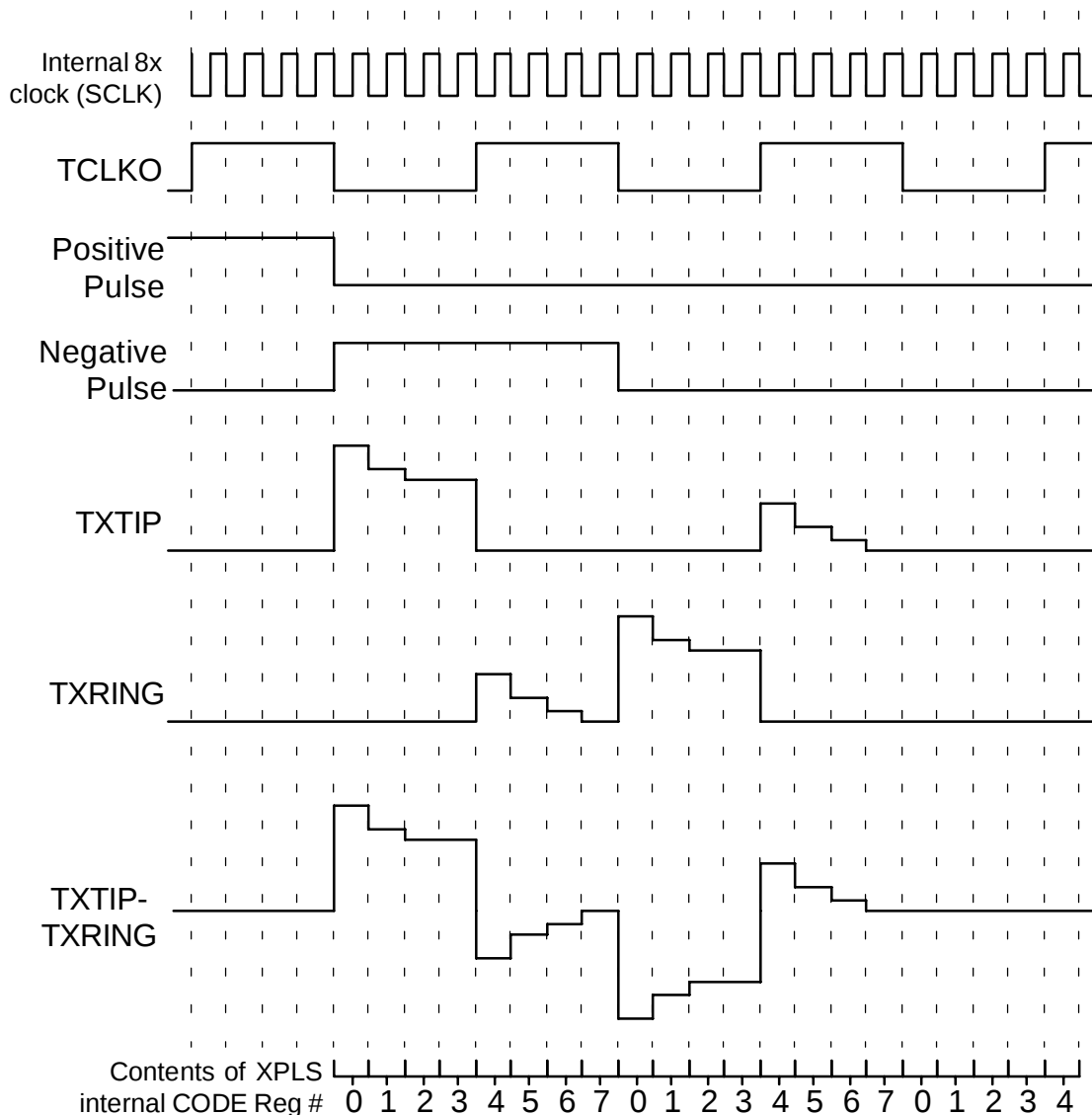
Figure 18 - CODE Register Sequence During Pulse Generation
