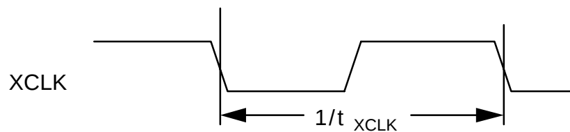
Figure 31 - XCLK Input Timing for Jitter Attenuation
