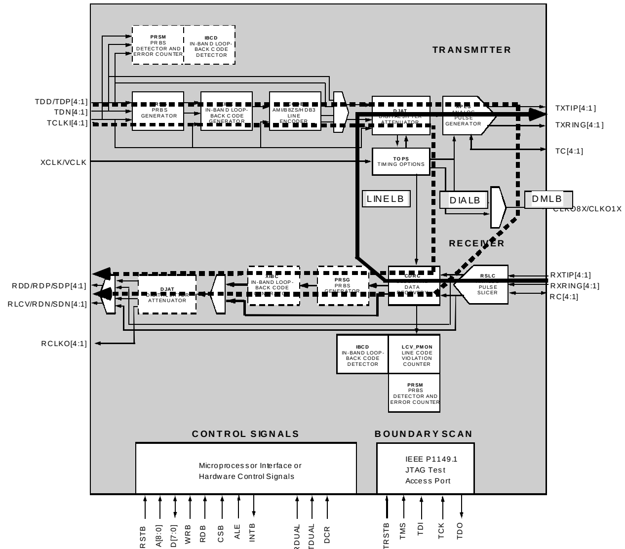
Figure 5 - Loopback Modes
