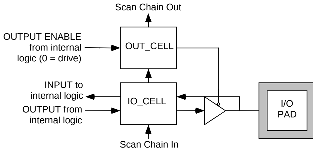
Figure 82 Layout of Output Enable and Bidirectional Cells
