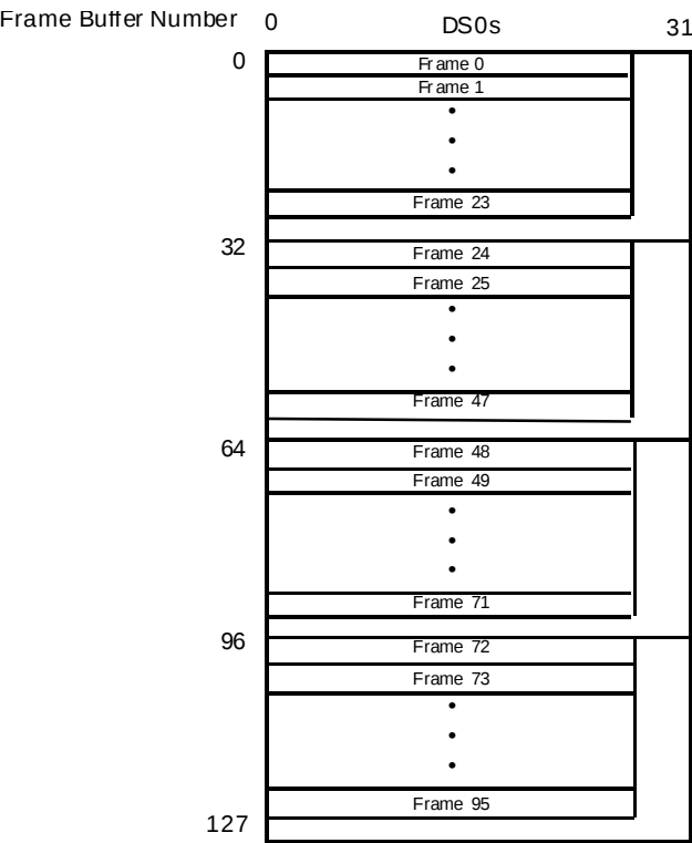
Figure 12 T1 SDF-FR Format of the T_DATA_BUFFER
