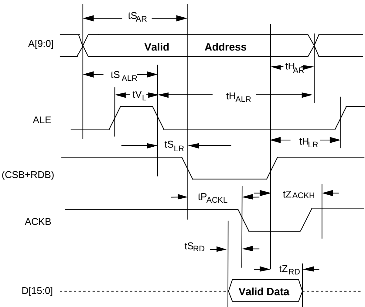
Figure 124 Microprocessor Interface Read Timing
