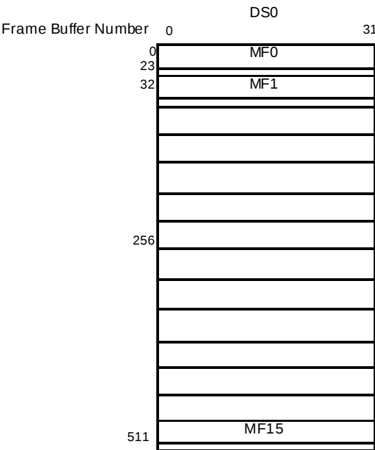
Figure 42 E1 SDF-MF with T1 Signaling Format of the R_DATA_BUFFER
