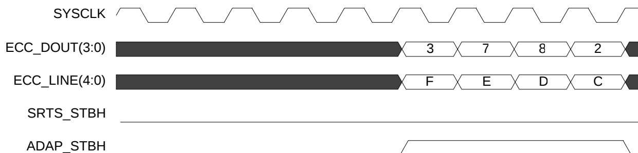
Figure 106 Channel Status Functional Timing
