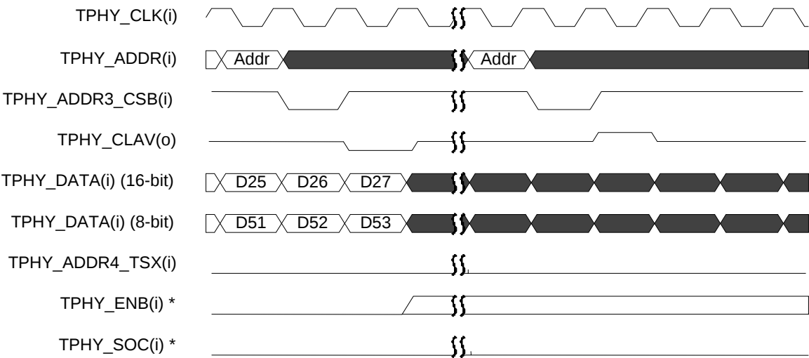
Figure 100 SNK_INTF End-of-Transfer (Any-PHY PHY Mode)
