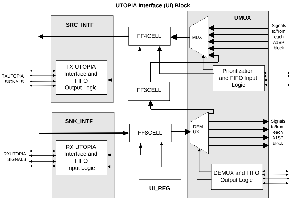
Figure 5 UI Block Diagram
