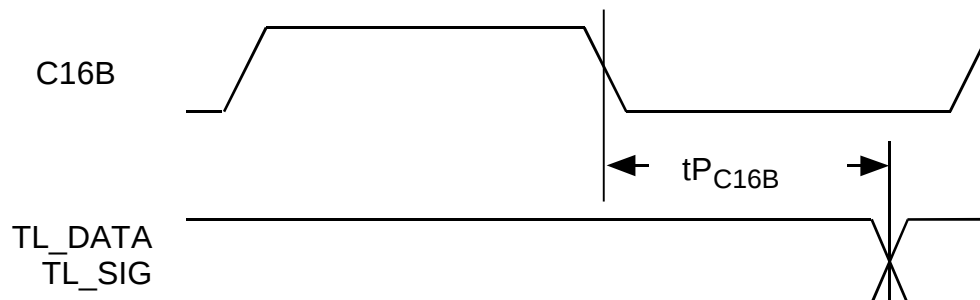
Figure 133 H-MVIP Ingress Data Timing
