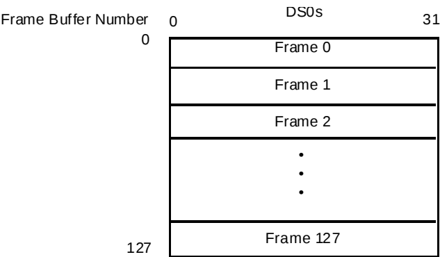
Figure 15 E1 SDF-FR Format of the T_DATA_BUFFER
