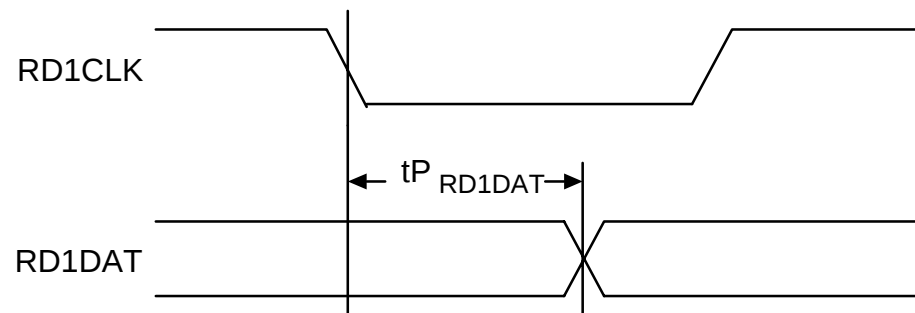
Figure 31 - Receive Tributary Output Timing
