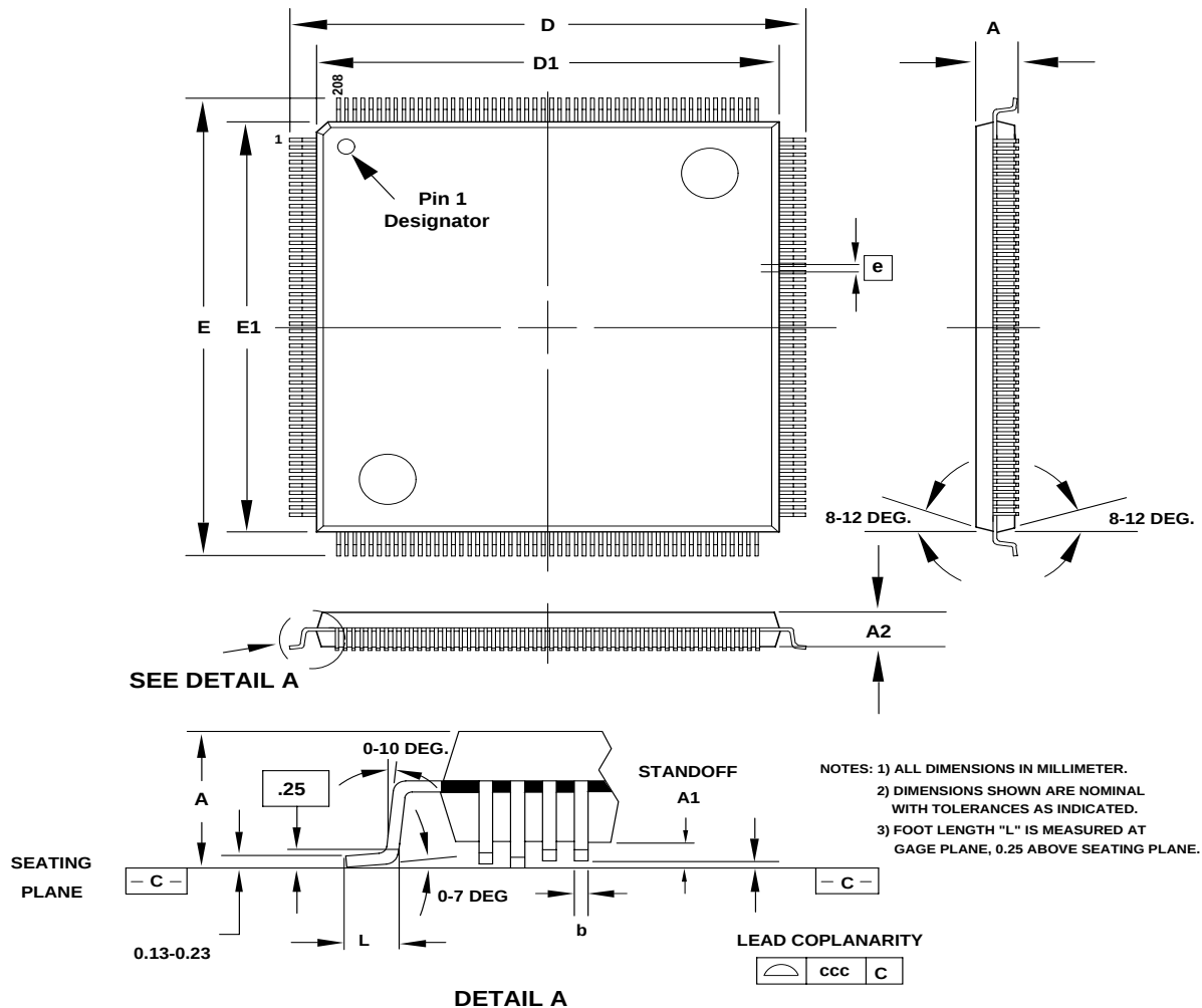
Figure 33 - 208 Pin Copper Leadframe Plastic Quad Flat Pack (R Suffix):
