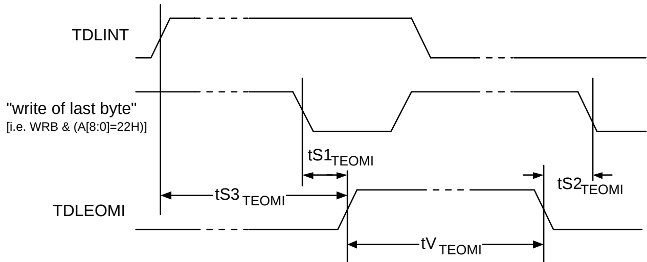
Figure 26 - Transmit Data Link EOM Input Timing
