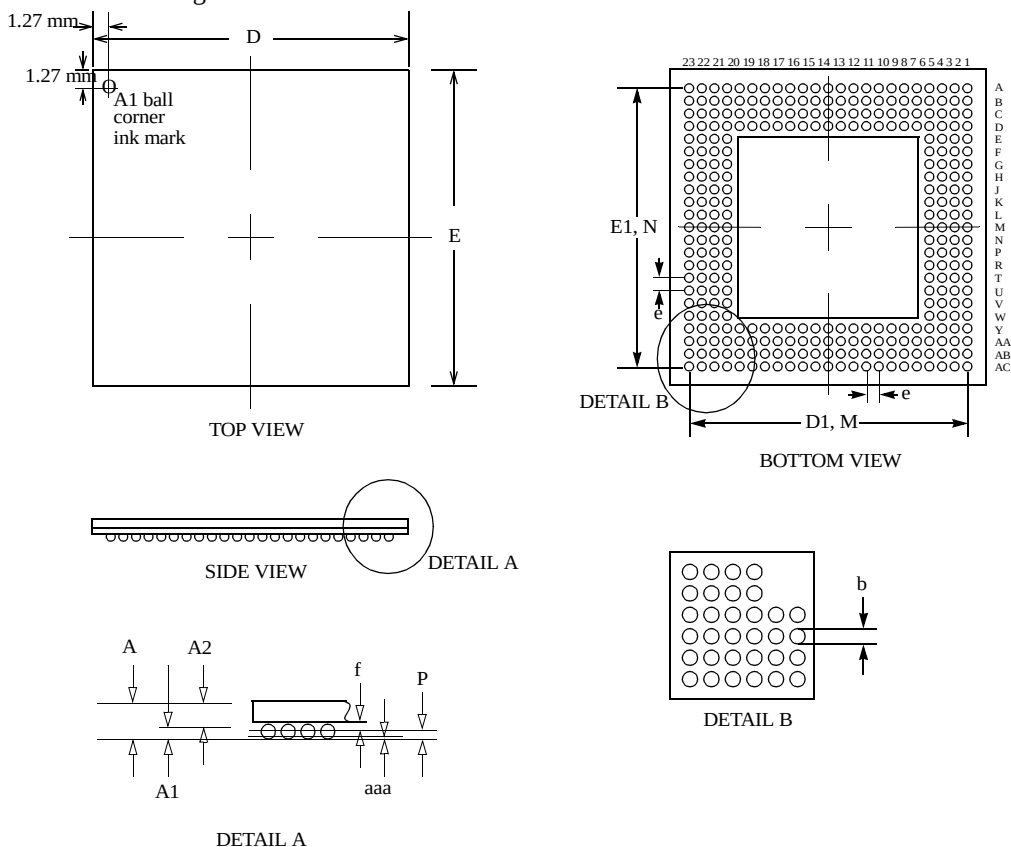
304 TBGA Drawing
