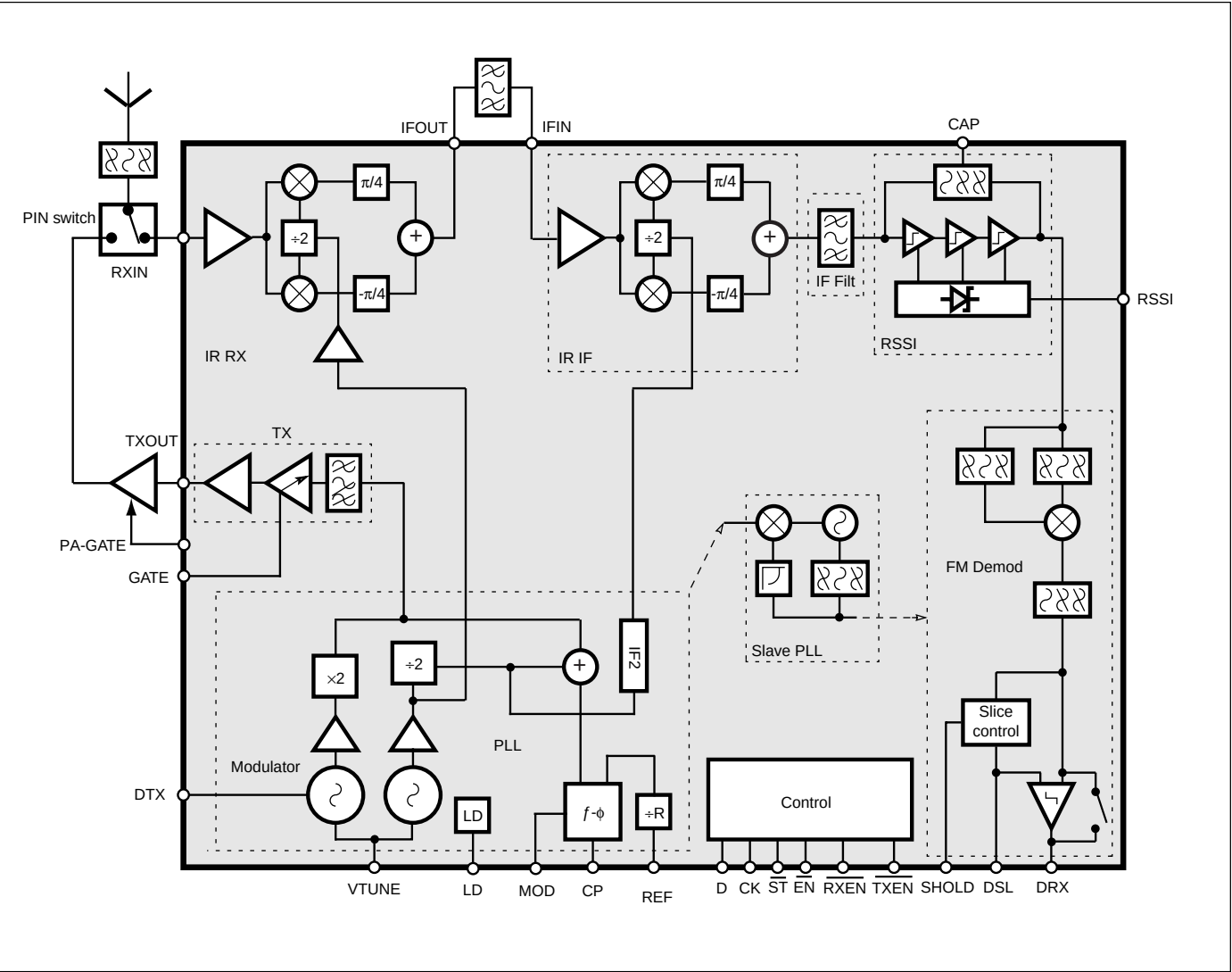
Figure 6. Block diagram.
