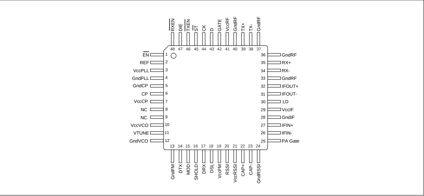
Figure 5. Pinning configuration.
