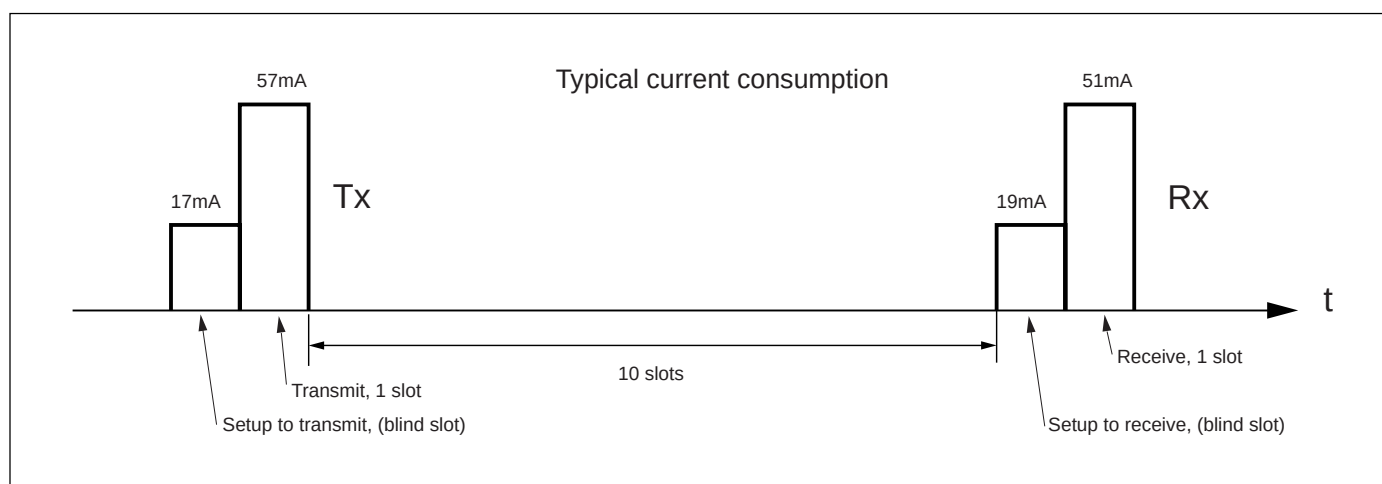
Figure 7. Typical current consumption.
