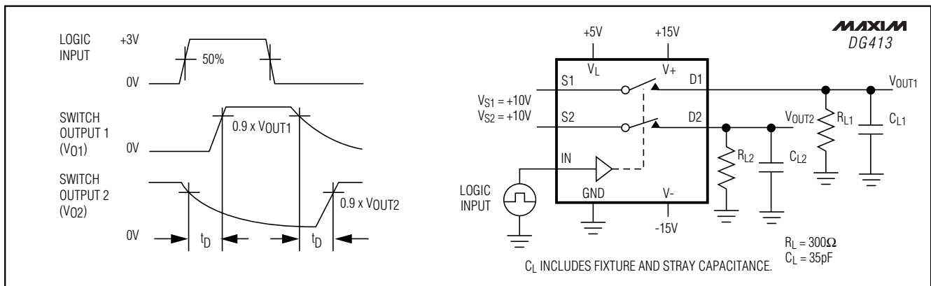
Figure 3. DG413 Break-Before-Make
