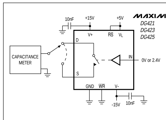
Figure 9. Drain/Source-On Capacitance
