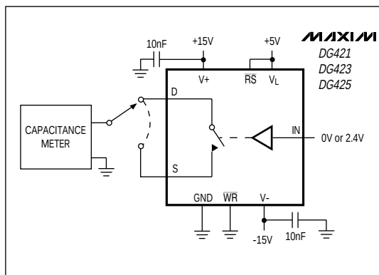
Figure 8. Drain/Source-Off Capacitance
