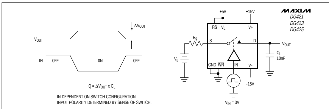
Figure 5. Charge Injection
