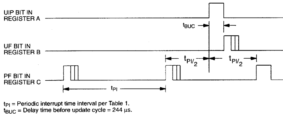
Figure 3. UPDATE-ENDED AND PERIODIC INTERRUPT RELATIONSHIP
