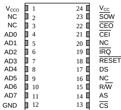
DS14287 24-Pin Encapsulated Package
