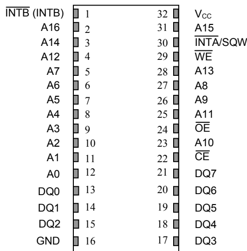
DS1486 128k x 8 32-Pin Encapsulated Package
