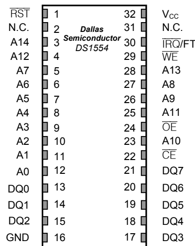
Encapsulated DIP
