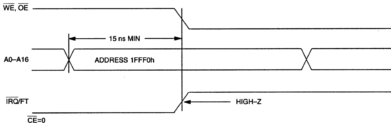
CLEARING IRQ WAVEFORMS Figure 3
