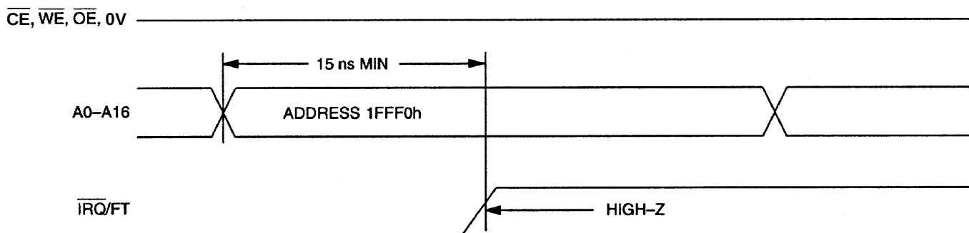
CLEARING IRQ WAVEFORMS Figure 3
