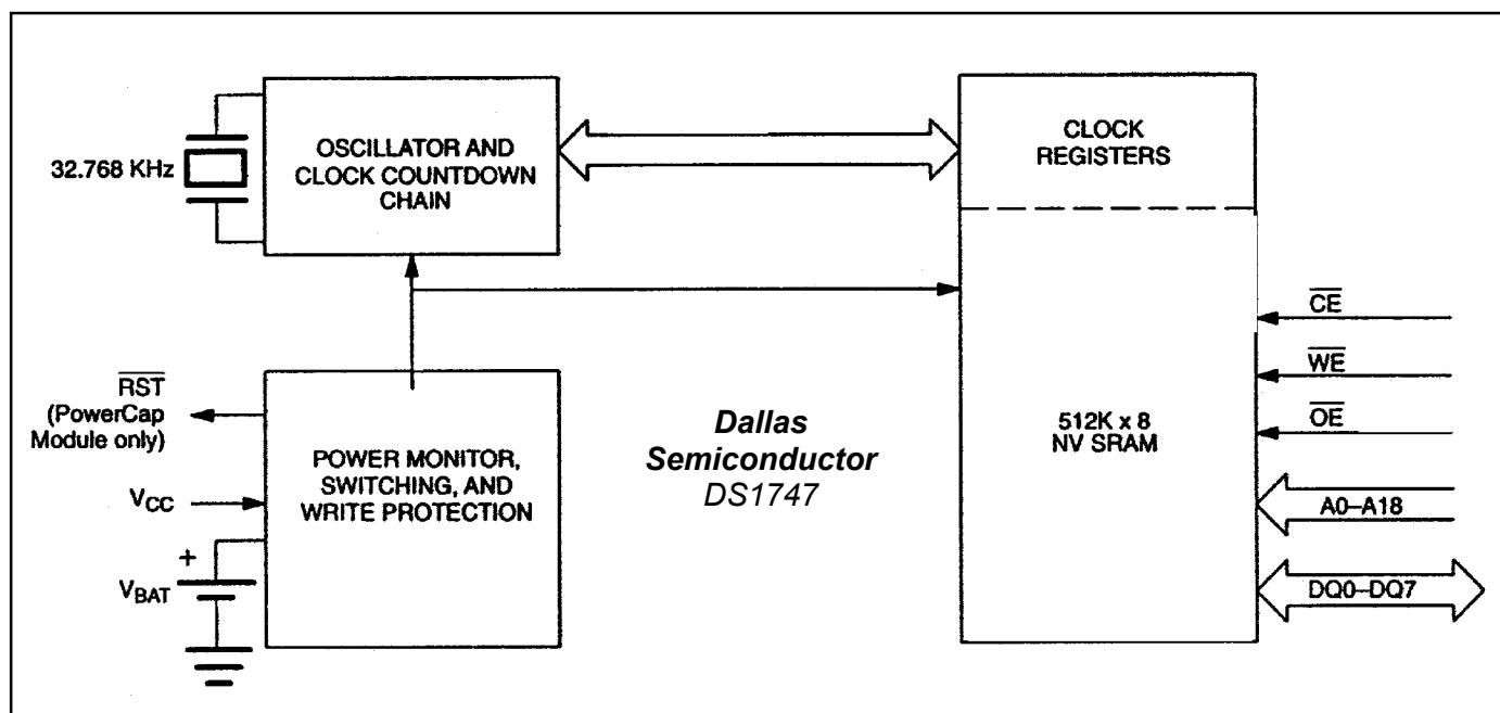
Figure 1. Block Diagram
