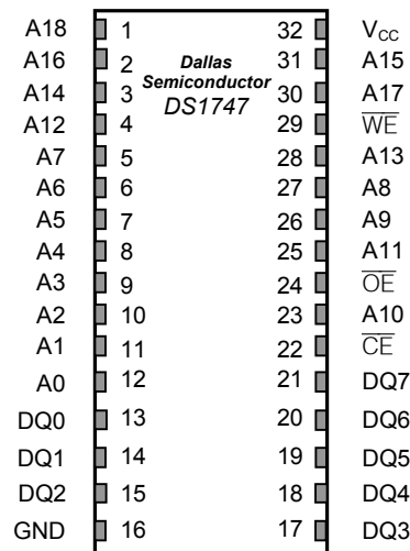
Encapsulated DIP (512k x 8)
