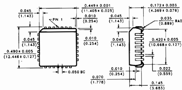
28 Lead Cerdip (JI) \theta_{JA} = 55^{\circ}\text{C/W}
