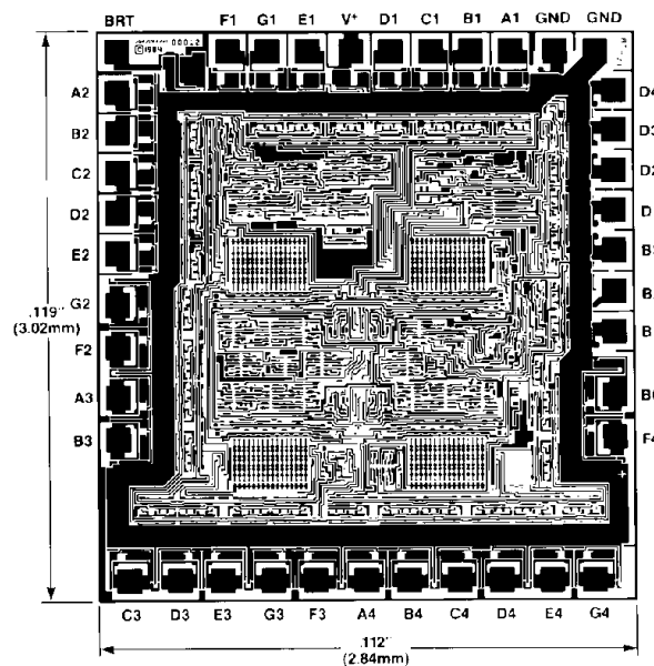
ICM7212, 12A
