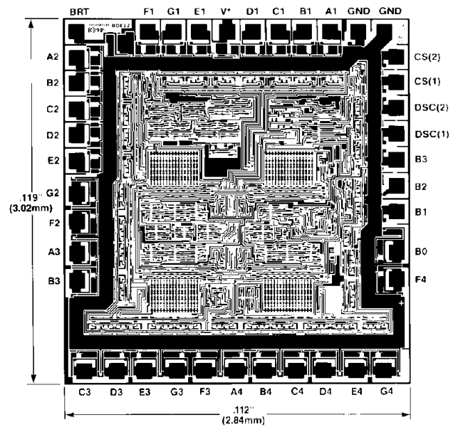
ICM7212M, 7212AM
