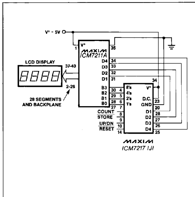
Figure 20. ICM7217 to LCD Interface.
