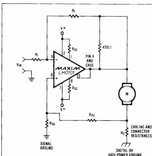
Figure 8. Correcting for Voltage Difference between Signal and Power Grounds.
