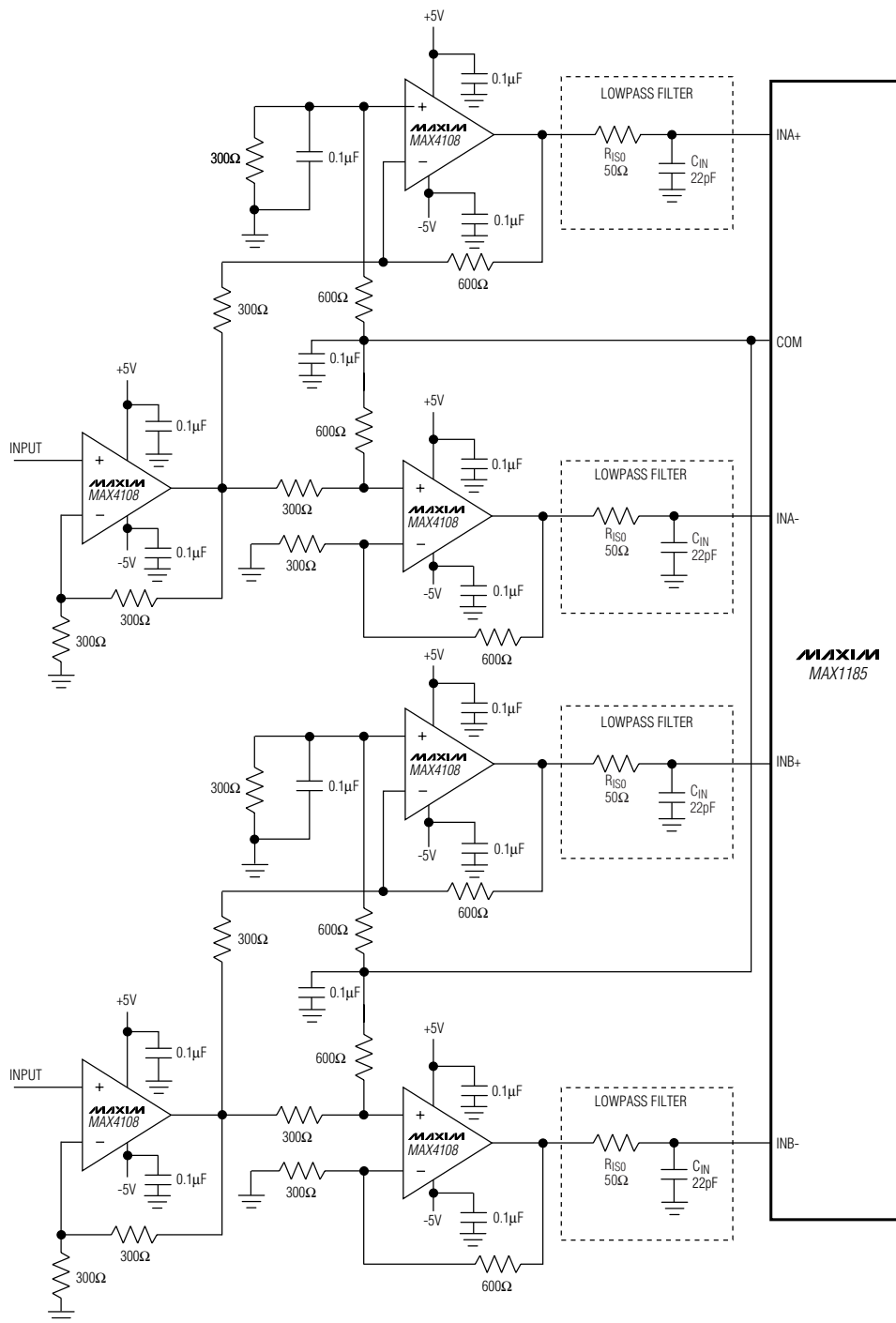
Figure 5. Typical Application for Single-Ended to Differential Conversion
