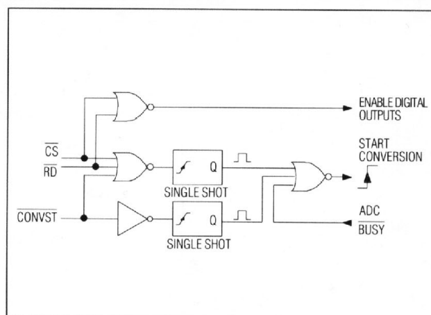
Figure 12. Conversion-Control Logic
