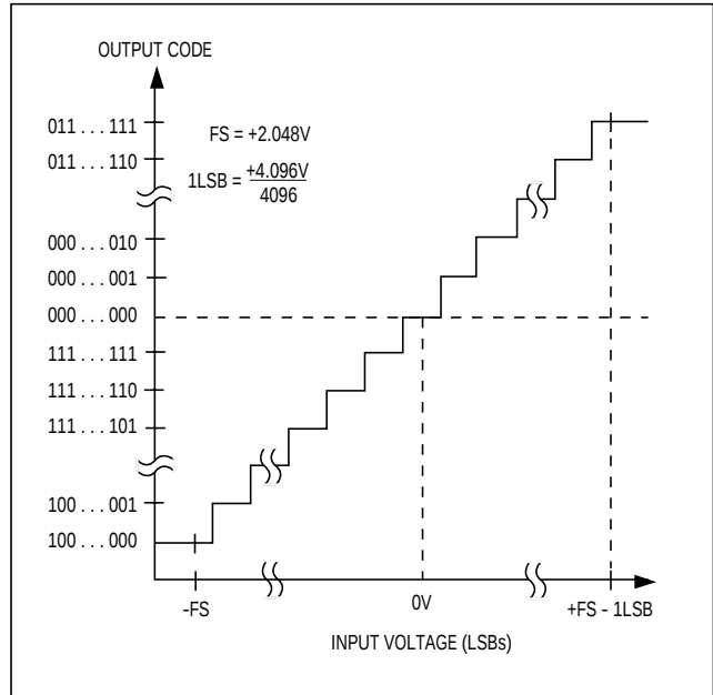
Figure 16. Bipolar Transfer Function, \pm 4.096\text{V}/2 = \text{Full Scale}
