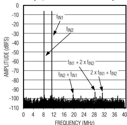
TWO-TONE FFT PLOT (16,384-POINT DATA RECORD)
