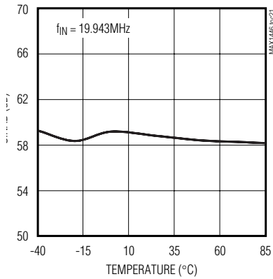
SIGNAL-TO-NOISE PLUS DISTORTION vs. TEMPERATURE
