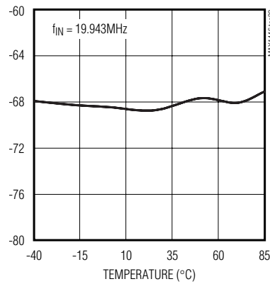
TOTAL HARMONIC DISTORTION vs. TEMPERATURE
