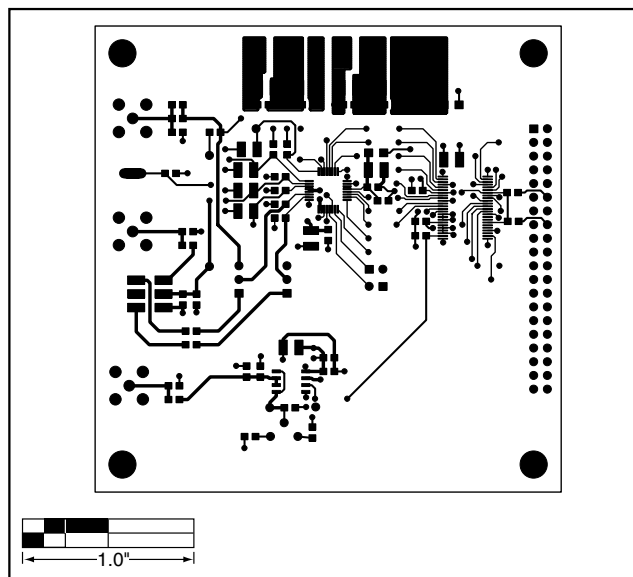
Figure 3. MAX1448EV Kit PC Board Layout—Component Side
