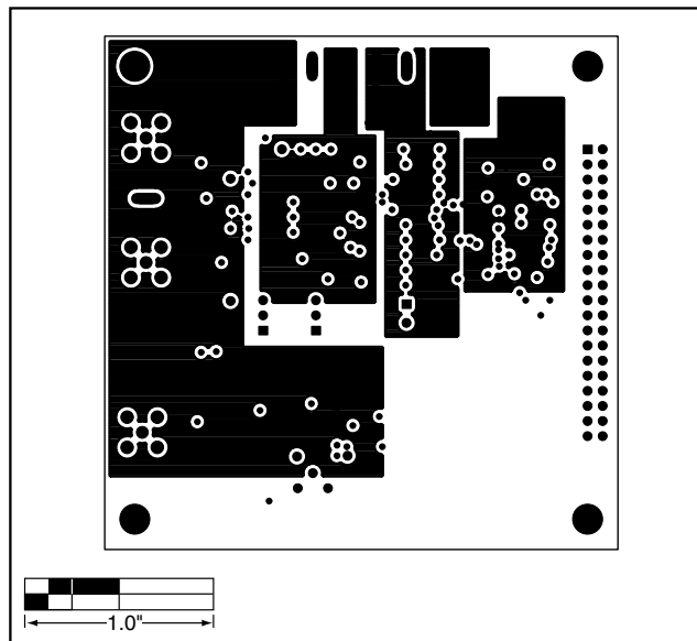
Figure 7. MAX1448EV Kit PC Layout—Power Planes
