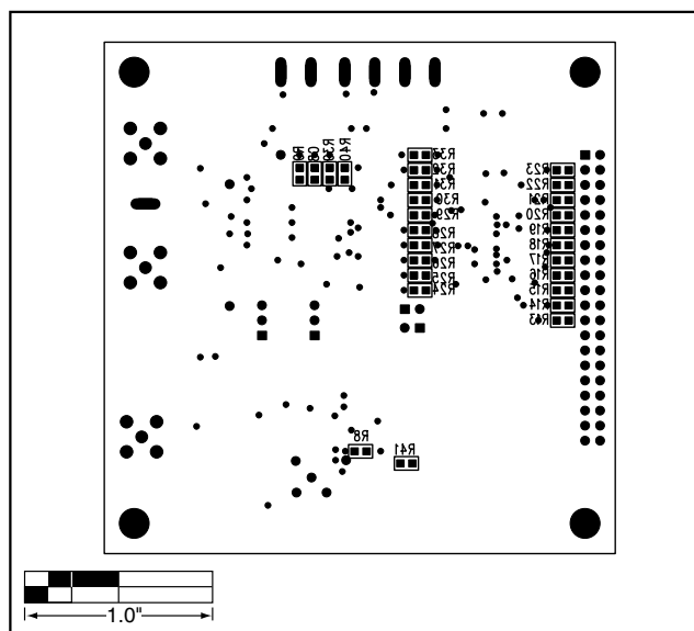
Figure 5. MAX1448EV Kit Component Placement Guide—Solder Side
