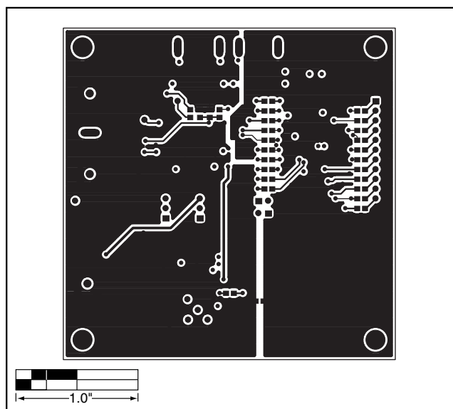
Figure 4. MAX1448EV Kit PC Board Layout—Solder Side
