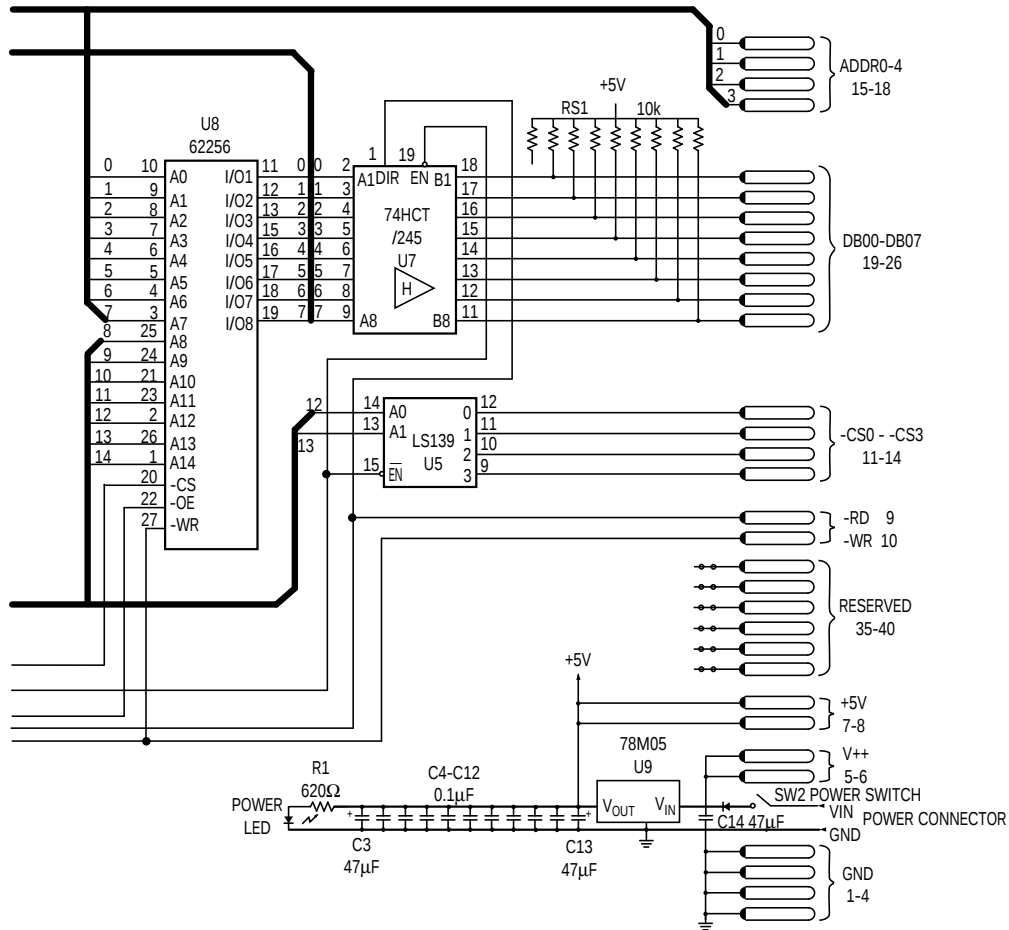
Figure 2. 80C32 Module Schematic (continued)
