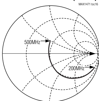
S11 SMITH CHART OF RFIN (434MHz)
