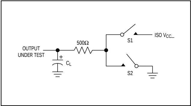
Figure 6. Driver Timing Test Load
