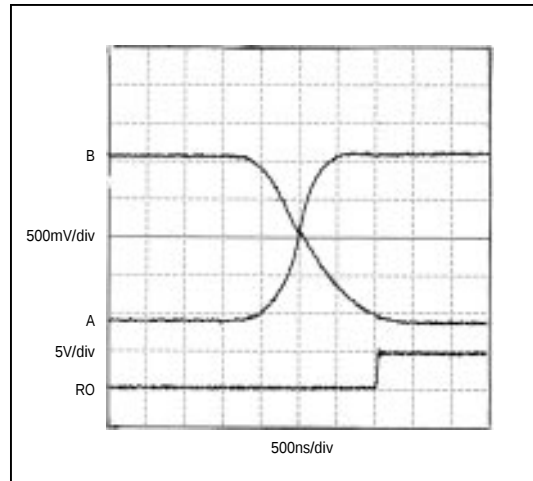
Figure 12. Receiver t_{PLH}
