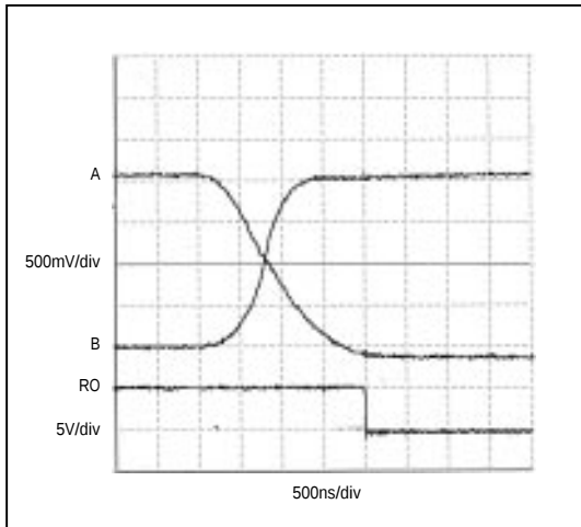
Figure 11. Receiver t_{PHL}
