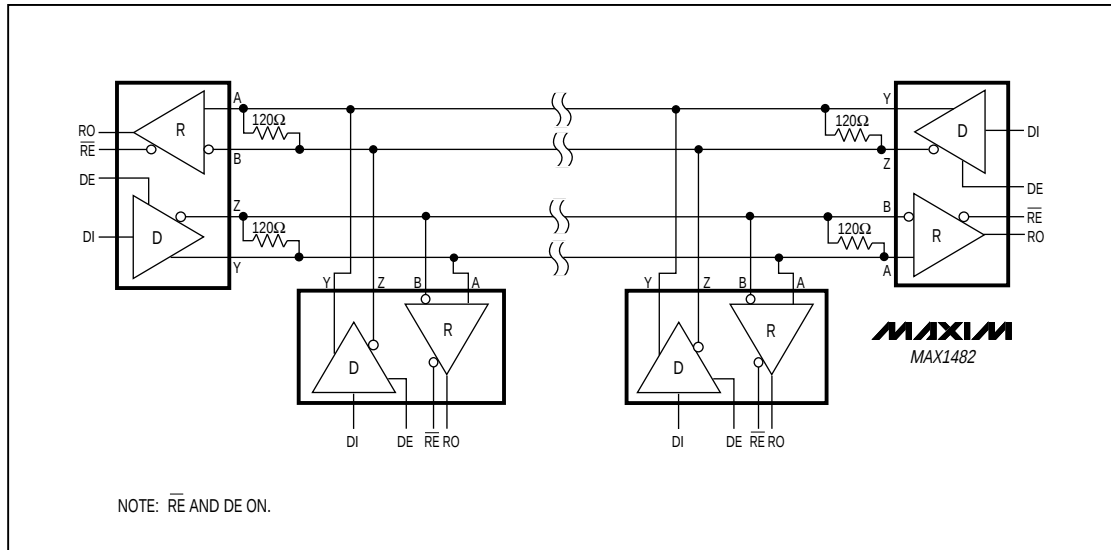
Figure 15. MAX1482 Full-Duplex RS-485 Network
