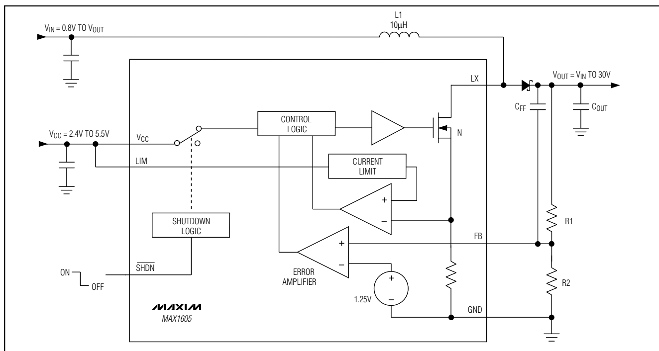
Figure 1. Functional Diagram
