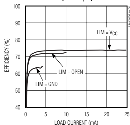
EFFICIENCY vs. LOAD CURRENT ( L1 = 10\mu H )
