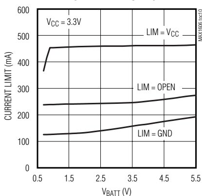
PEAK INDUCTOR CURRENT LIMIT vs. BATTERY VOLTAGE
