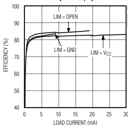
EFFICIENCY vs. LOAD CURRENT ( L1 = 100\mu H )
