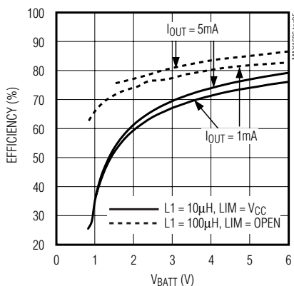
EFFICIENCY vs. BATTERY VOLTAGE
