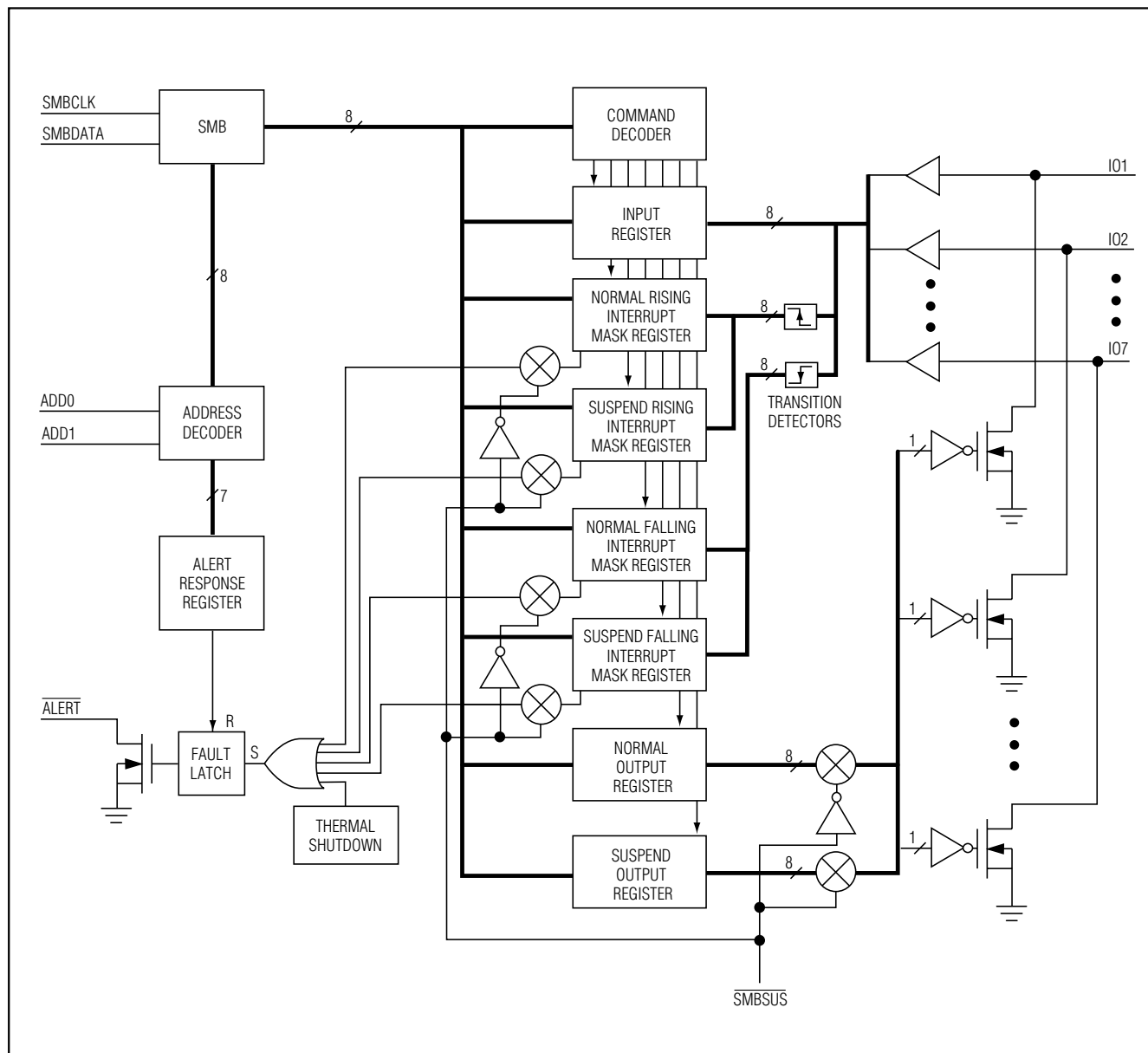
Figure 1. Functional Diagram
