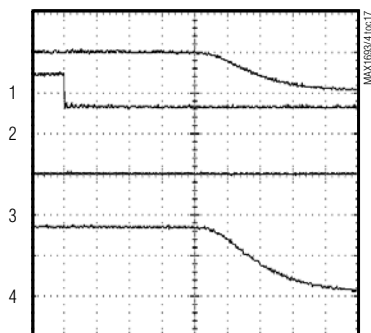
MAX1693H SWITCH TURN-OFF TIME
