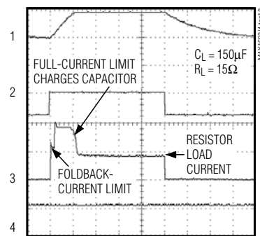
MAX1693H STARTUP TIME (TYPICAL USB APPLICATION)
