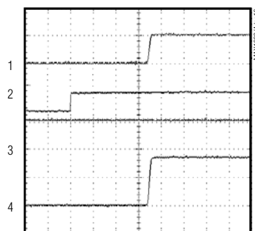
MAX1693H SWITCH TURN-ON TIME
