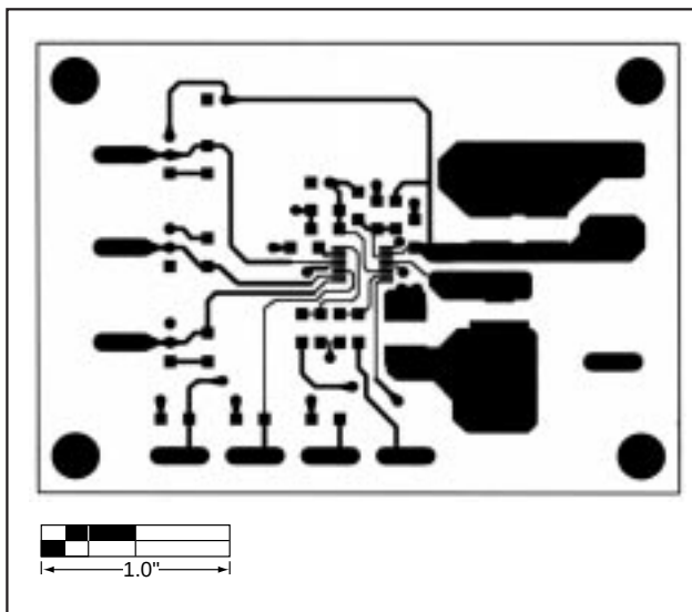
Figure 3. MAX1701 EV Kit PC Board Layout—Component Side
