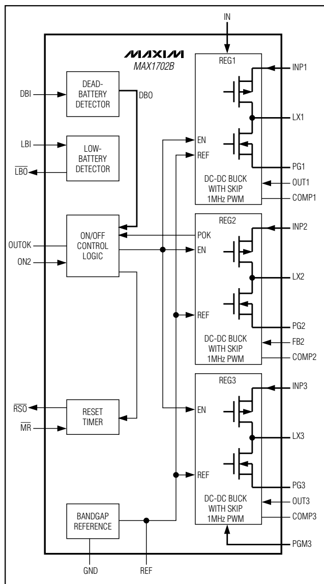
Functional Diagram
