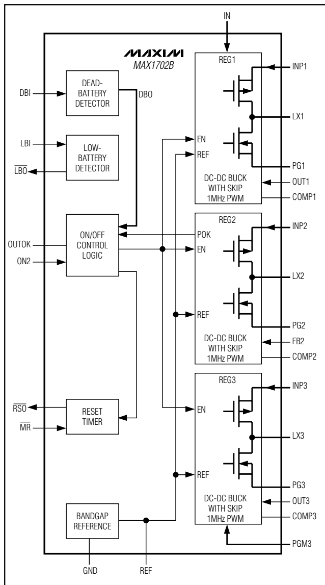
Functional Diagram
