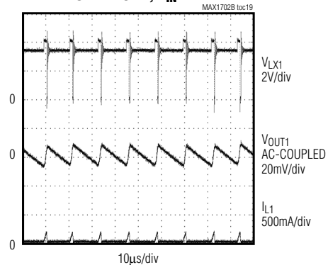
REG1 LIGHT-LOAD SWITCHING WAVEFORM LOAD = 10mA, V_{IN} = 4V
