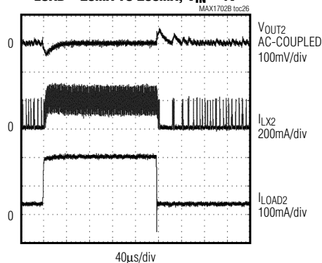
REG2 LOAD TRANSIENT WAVEFORM LOAD = 20mA TO 200mA, V_{IN} = 4\text{V}
