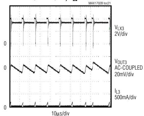
REG3 LIGHT-LOAD SWITCHING WAVEFORM LOAD = 10mA, V_{IN} = 4V
