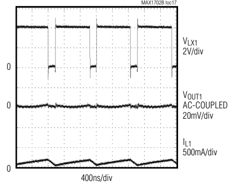
REG1 MEDIUM-LOAD SWITCHING WAVEFORM LOAD = 100mA, V_{IN} = 4V
