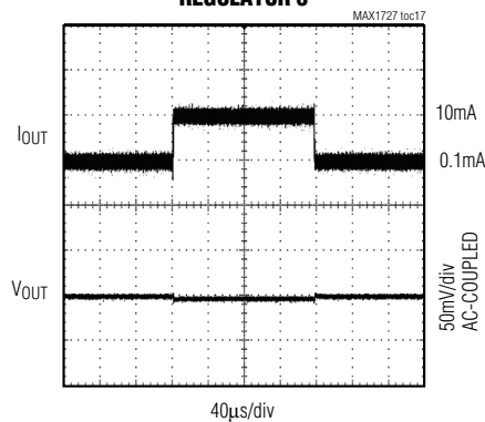
LOAD-TRANSIENT RESPONSE REGULATOR 3
