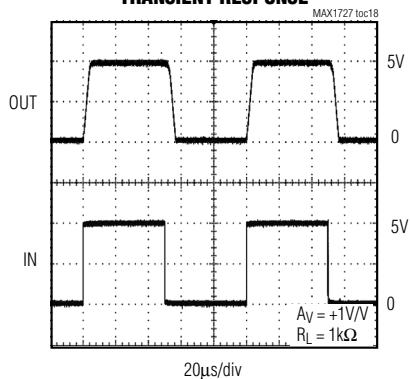
OP AMP LARGE-SIGNAL TRANSIENT RESPONSE
