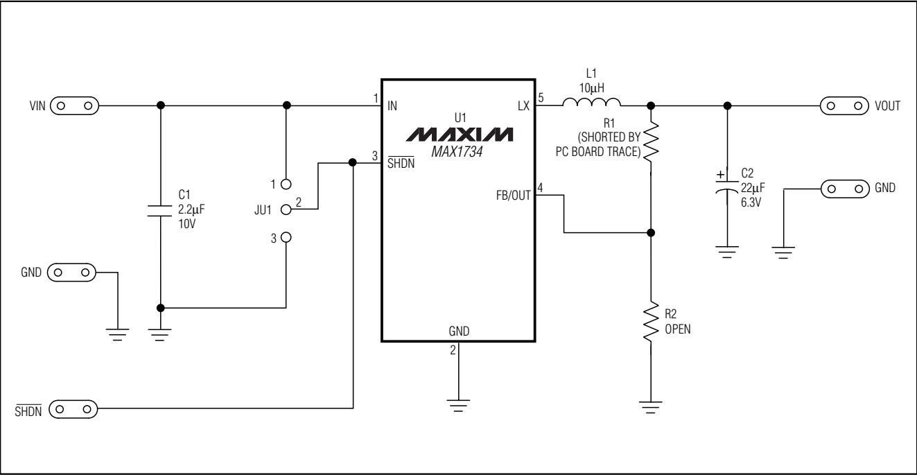
Figure 1. MAX1734 EV Kit Schematic
