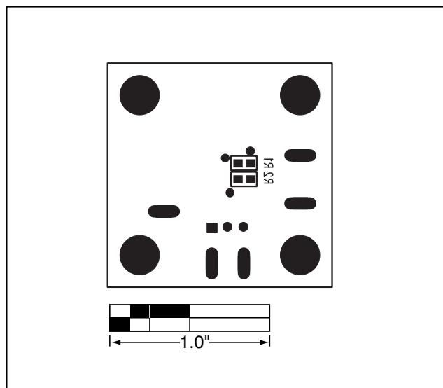
Figure 3. MAX1734 EV Kit Component Placement Guide—Solder Side
