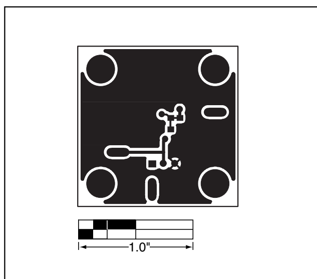
Figure 5. MAX1734 EV Kit PC Board Layout—Solder Side
