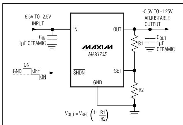
Figure 3. Typical Application Circuit with Adjustable Output Voltage
