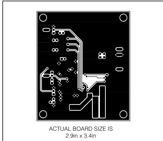
Figure 4. MAX1737 EV Kit PC Board Layout—Solder Side
