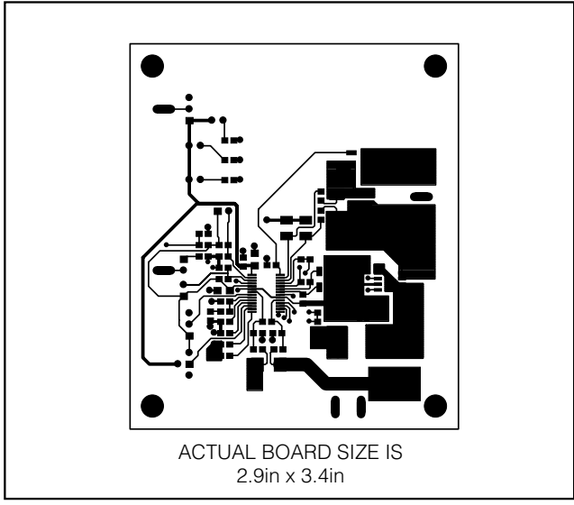
Figure 3. MAX1737 EV Kit PC Board Layout—Component Side
