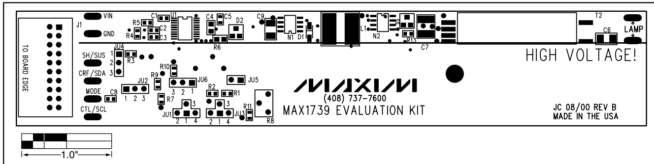
Figure 3. MAX1739 EV Kit Component Placement Guide—Component Side
