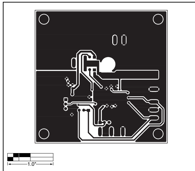
Figure 4. MAX1748 EV Kit PC Board Layout—Solder Side
