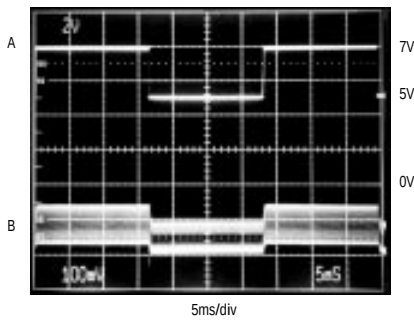
LINE-TRANSIENT RESPONSE
