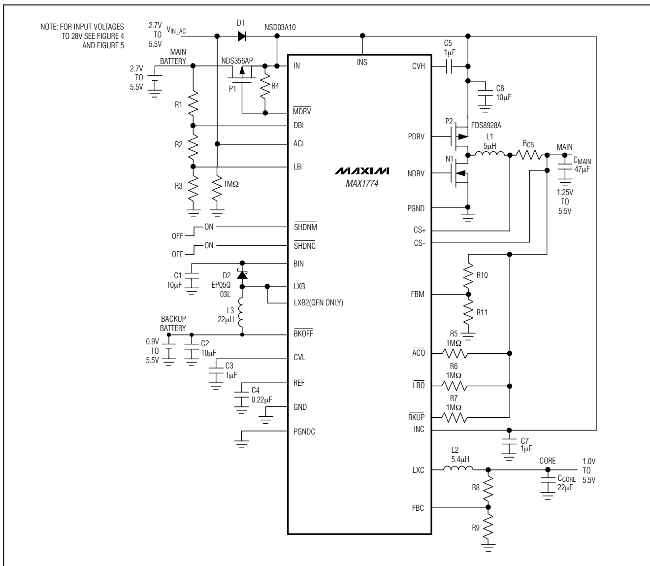
Figure 1. Typical Application Circuit For Low-Input Voltage Applications
