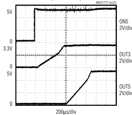
DELAYED START WAVEFORMS (ON3 = REF)
