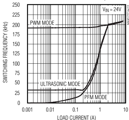
3.3V OUTPUT SWITCHING FREQUENCY vs. LOAD CURRENT (MAX1977)
