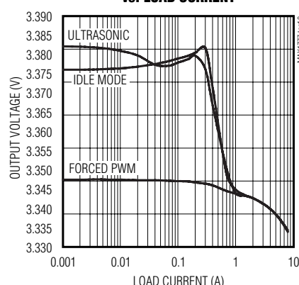
OUT3 VOLTAGE REGULATION vs. LOAD CURRENT
