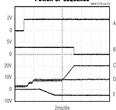
POWER-UP SEQUENCE
