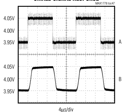
VCOM BUFFER SMALL-SIGNAL RESPONSE
