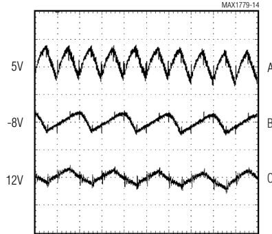
RIPPLE WAVEFORMS
