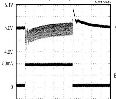
LOAD TRANSIENT (L = 10 μH, 500 μs PULSE)
